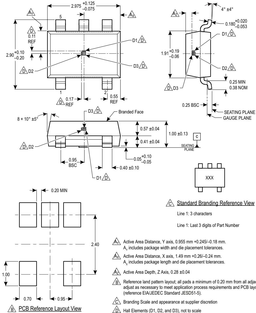
Figure 15: Package LH, 5-Pin SOT23-W
