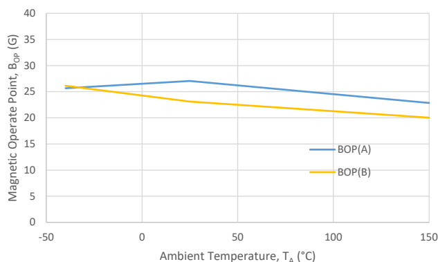
Operate Point vs. Temperature V_{DD} = 2.8\text{ V}
